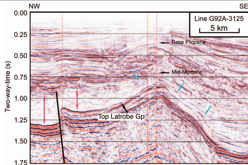
Figure 7 Seismic line G92A-3125 (see Figure 6 for location) offshore Gippsland Basin. Early Miocene sediments onlap (blue arrows) the deeper structure, indicating deformation within the Oligocene–Early Miocene. Onlapping reflectors, stratigraphic thinning and folding higher in the section indicate that deformation continued into the Plio-Pleistocene. Different stratigraphic thicknesses on either side of the reverse fault (red arrows) indicate fault movement within the Oligocene–Early Miocene (modified from Dickinson et al. 2001).
