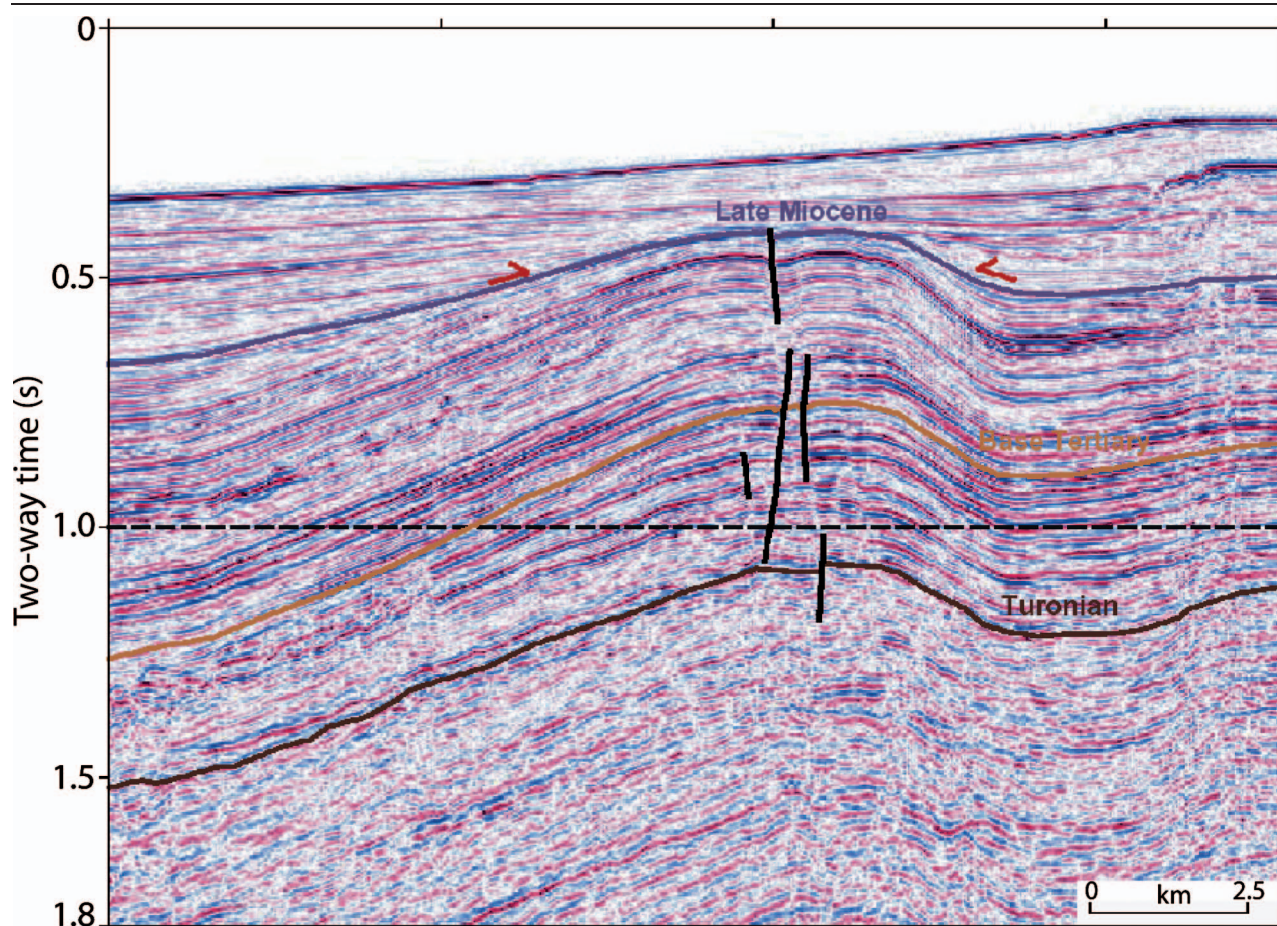
Figure 5 Miocene inversion structure over the Lombardina structure, Browse Basin, Northwest Shelf, AGSO seismic line 175/03 (modified from Struckmeyer et al. 1998, where a detailed interpretation of this structure can be found).
