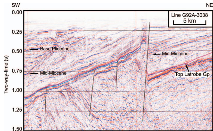
Figure 8 Seismic line G92A-3038 offshore Gippsland (see Figure 6 for location) showing relatively young (post-Middle Miocene) reverse movement on the Rosedale Fault System (modified from Dickinson et al. 2001).
