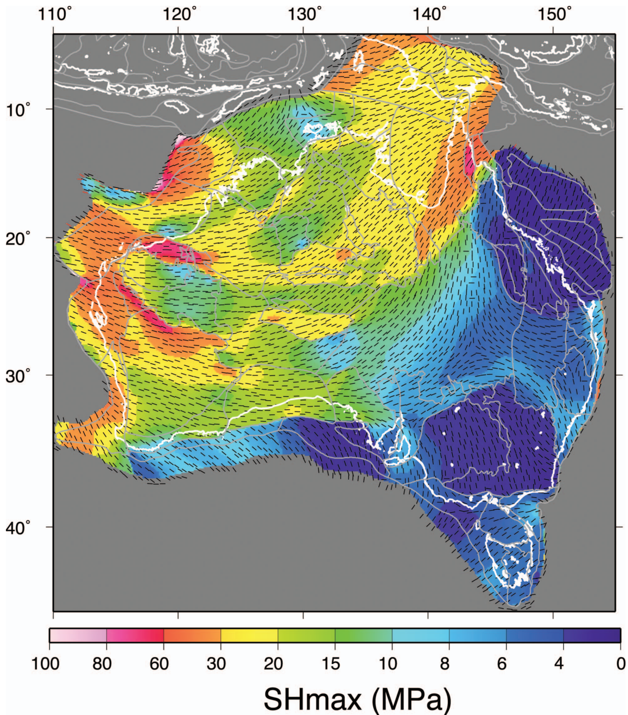
Figure 12 Modelled maximum horizontal stress for the Late Miocene (11–6 Ma). Stress magnitude units are in MPa.
