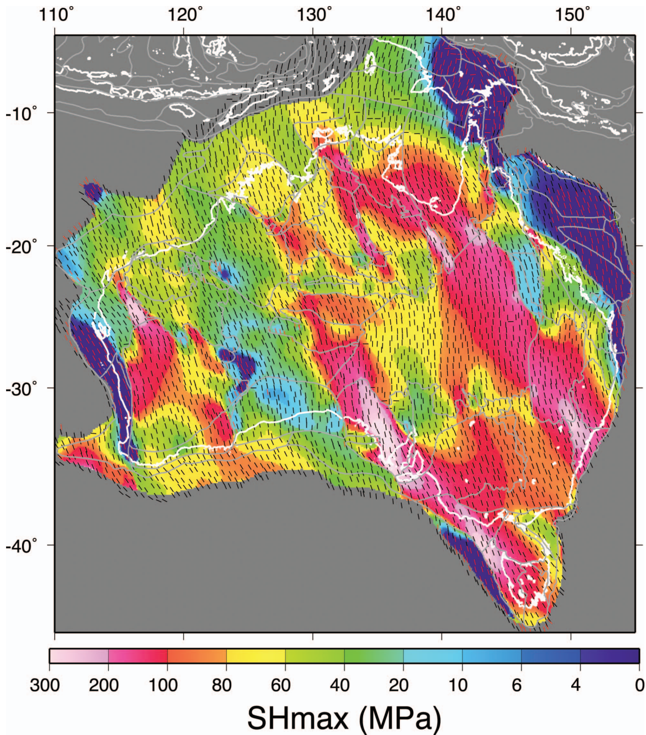
Figure 9 Modelled maximum horizontal stress for the Cretaceous ( ca 100 Ma). Stress magnitude units are in MPa.
