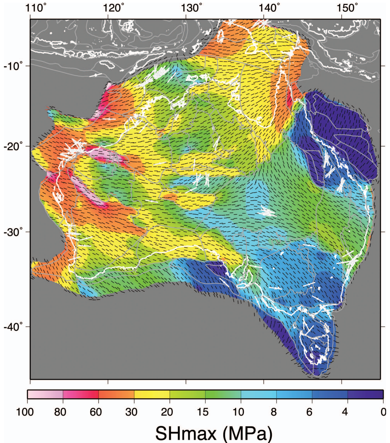
Figure 13 Modelled contemporary (6–0 Ma) maximum horizontal stress. Orientation data from the Australian Stress Map Database shown by white filled bars. Stress magnitude units are in MPa.
