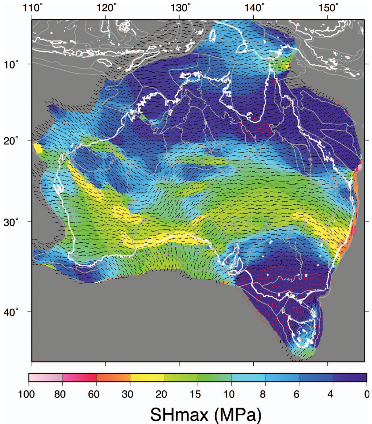
Figure 10 Modelled maximum horizontal stress for the Eocene ( ca 55 Ma). Stress magnitude units are in MPa.
